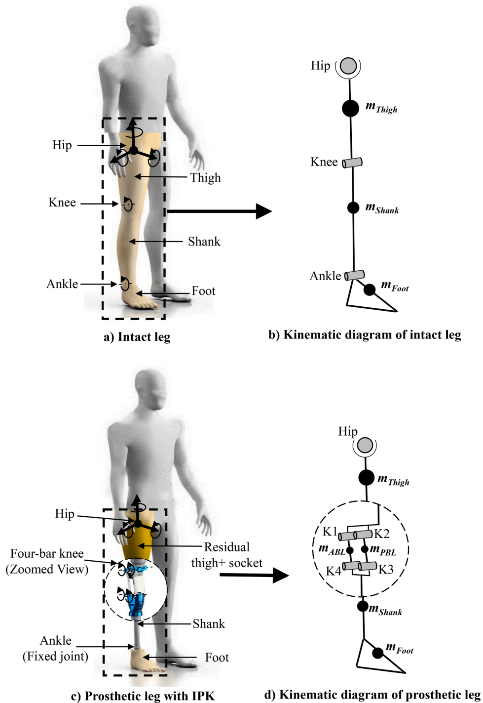
Fig. 2. Intact and prosthetic leg models used for 3D analyses.
